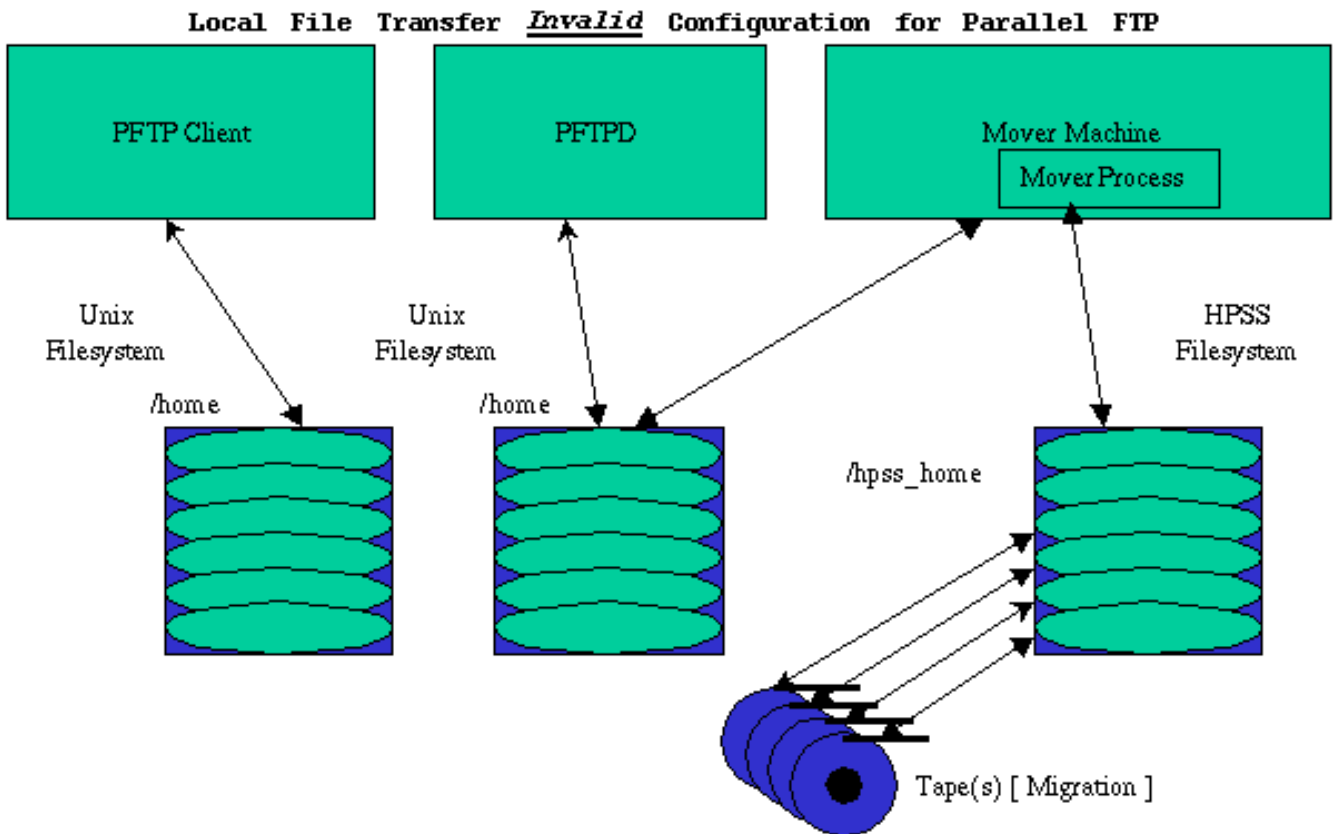
Figure 3. Local file transfer invalid configuration for PFTP
