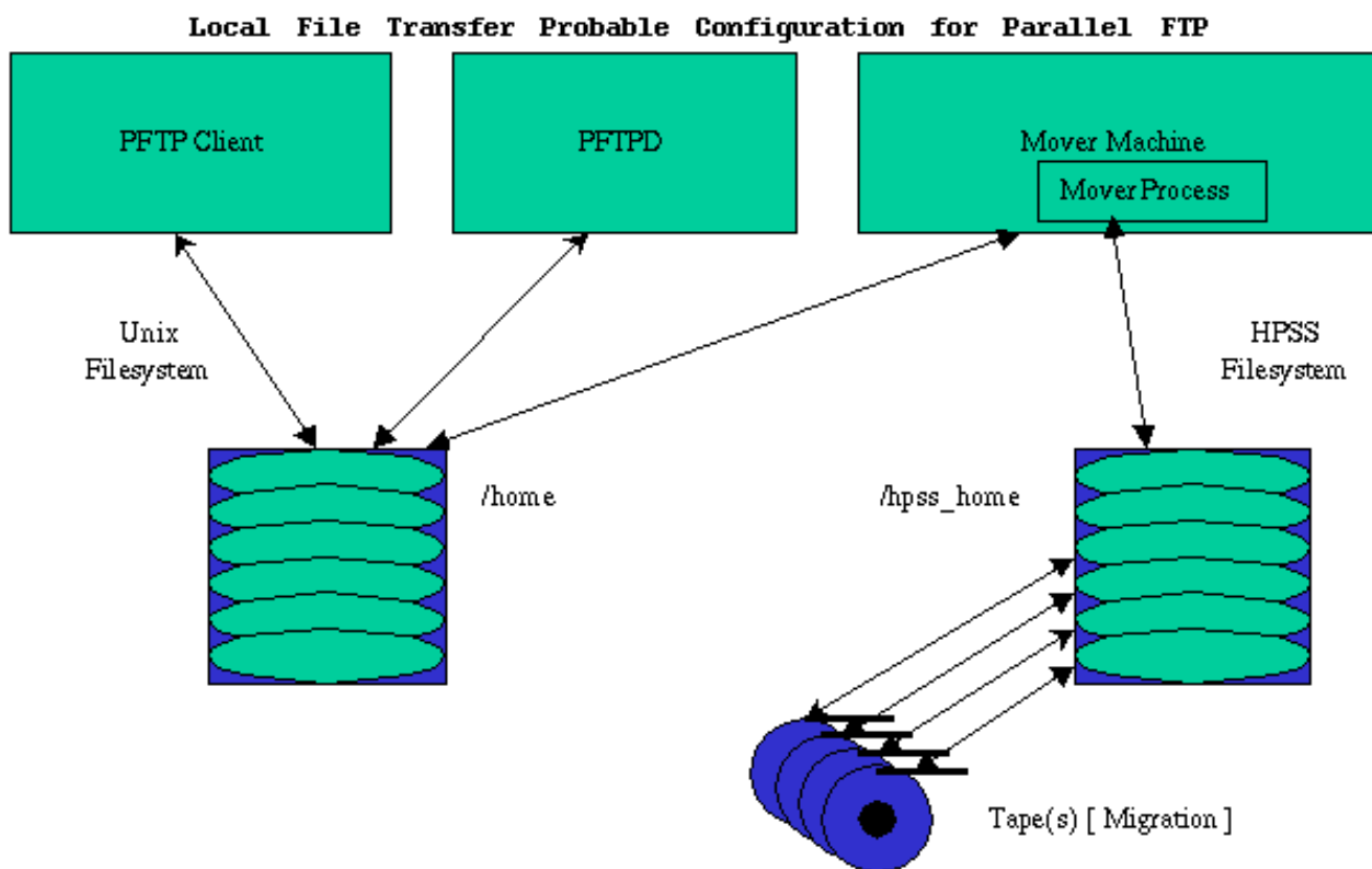
Figure 1. Local File Transfer Probable Configuration for PFTP
