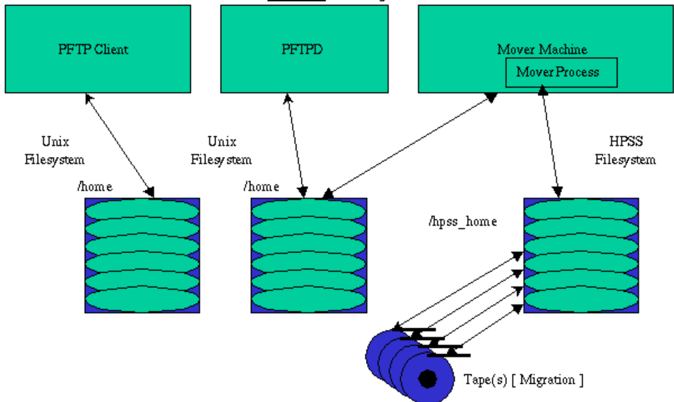
Figure 3. Local file transfer invalid configuration for PFTP
